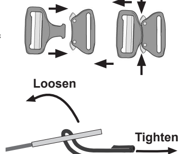
fig 2 - Fastening Quick Connect Buckles
